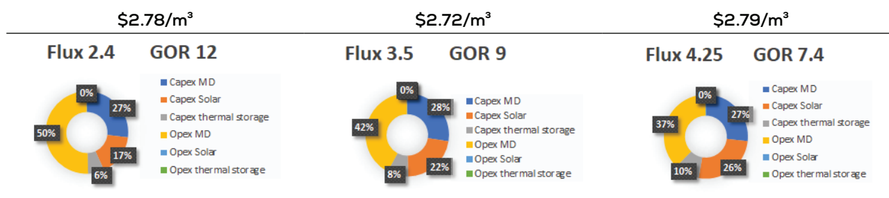
Figure 2. COW for 3 different operational conditions with the same boundary conditions: Costs of water for different Key Performance Indicators FLUX (liters / m² of membrane per hour) GOR (x times more energy efficient compared to 'normal' evaporation)
